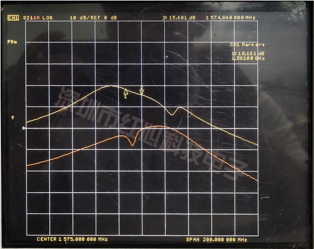
(Gain)增益图
