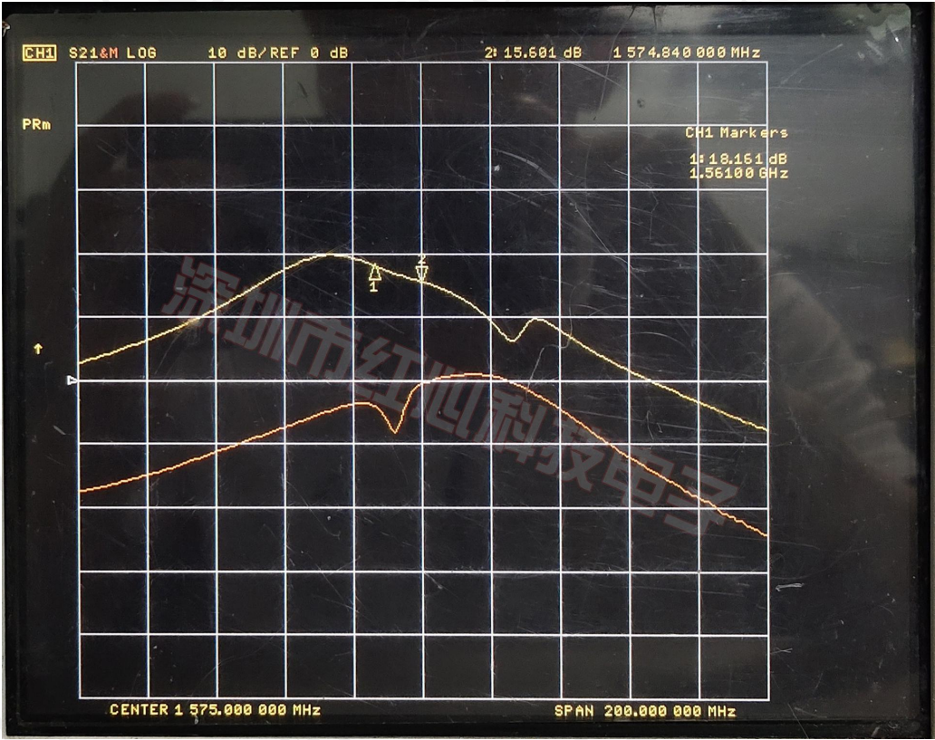
(Gain)增益图
